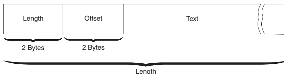
Figure 2. Format of the Command Buffer
