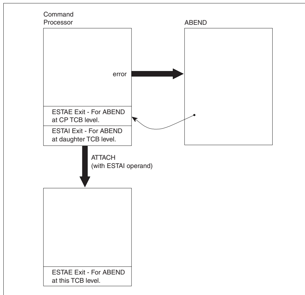
Figure 12. ABEND, ESTAI, ESTAE Relationship
