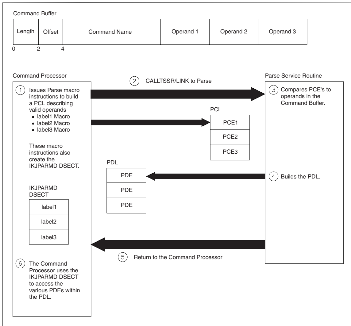
Figure 4. A Command Processor Using the Parse Service Routine
